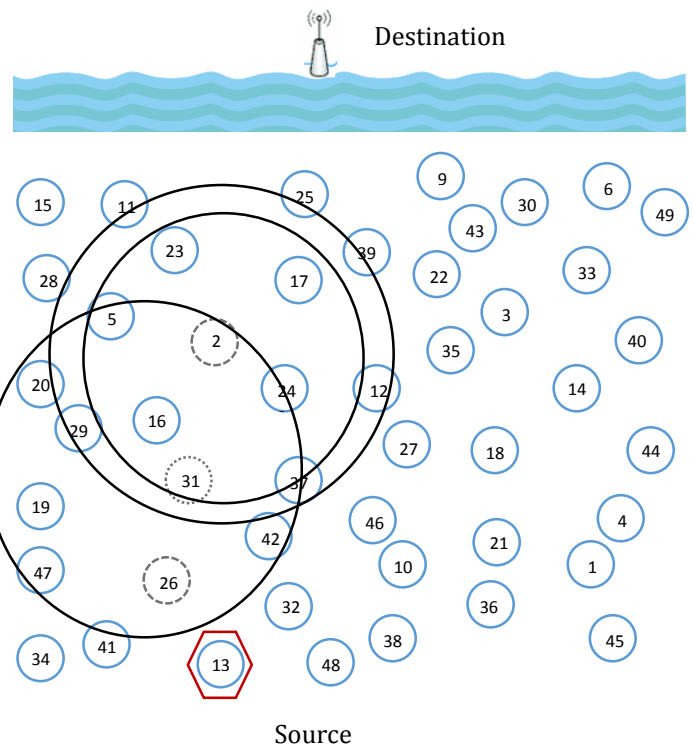
Fig -3: Search for the best path in improved ACO algorithm
