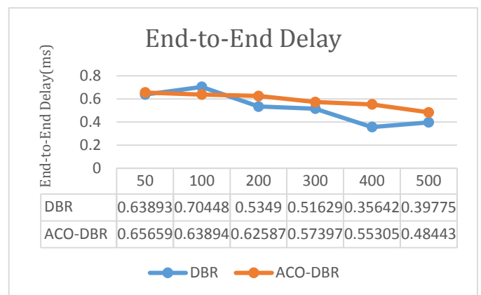
Chart -3: End-to- End Delay vs. Number of Nodes.
