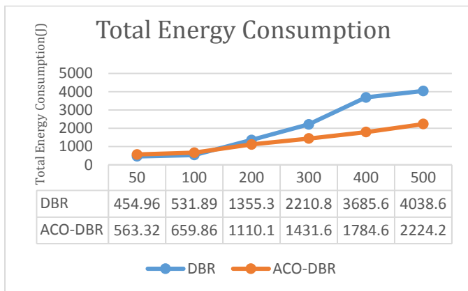
Chart -1: Total Energy Consumption vs. Number of Nodes.
